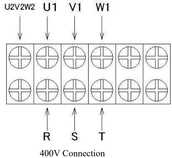
Circuit drawing for each voltage
