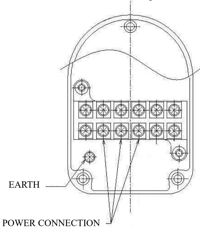
Terminal Diagram
