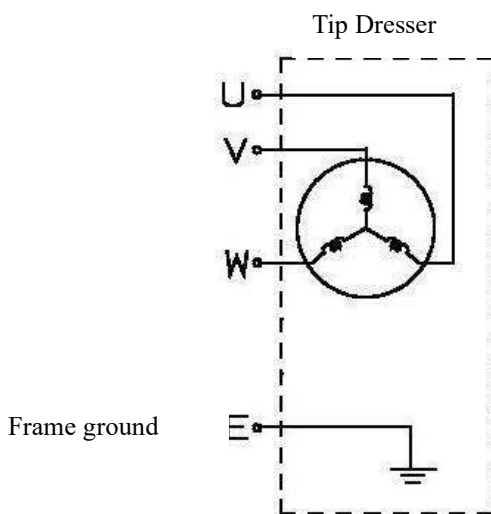
Motor circuit diagram
